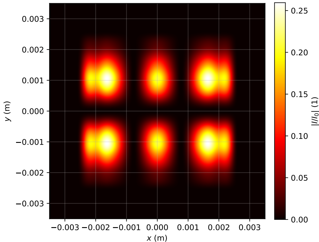
Intensity profile I(x, y, z = 3.821)/I_0 , P_{in}=1.0P_{cr} , artificial time
